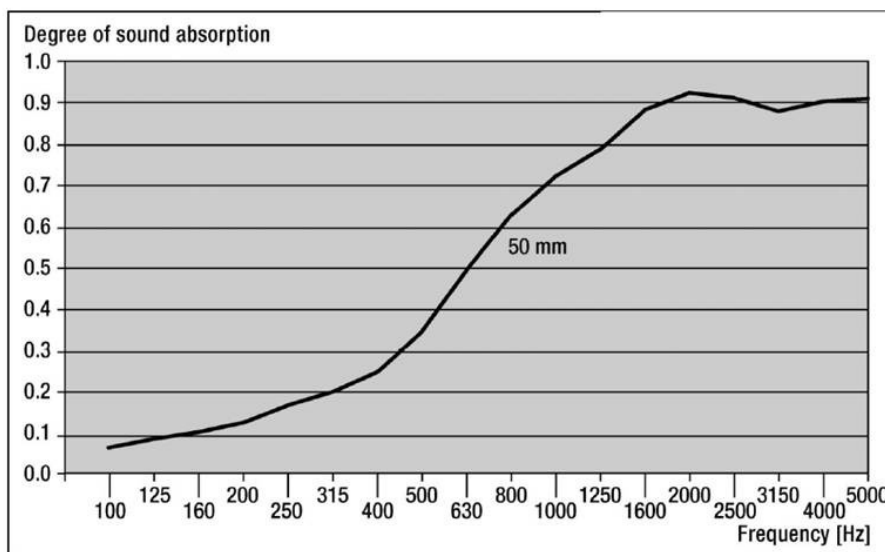
Sound absorption according to ISO 10534-2
